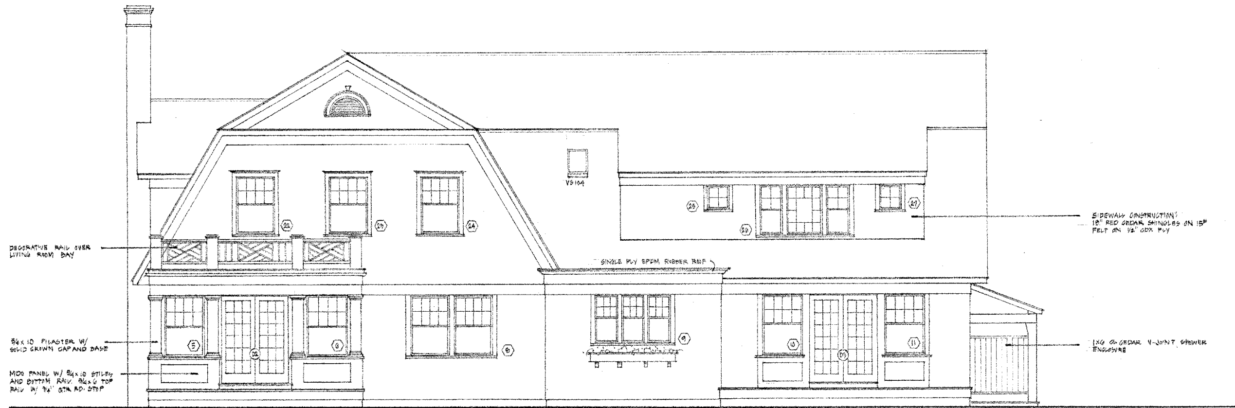
SOUTH ELEVATION 1/4" = 1'-0"
